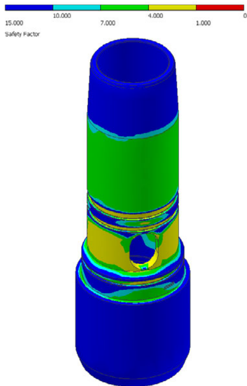
Figure 6.3 2-7/8: Safety Factor at 2810 ft-lb Cooler colours indicate higher safety factor. Red areas indicate yielding.
