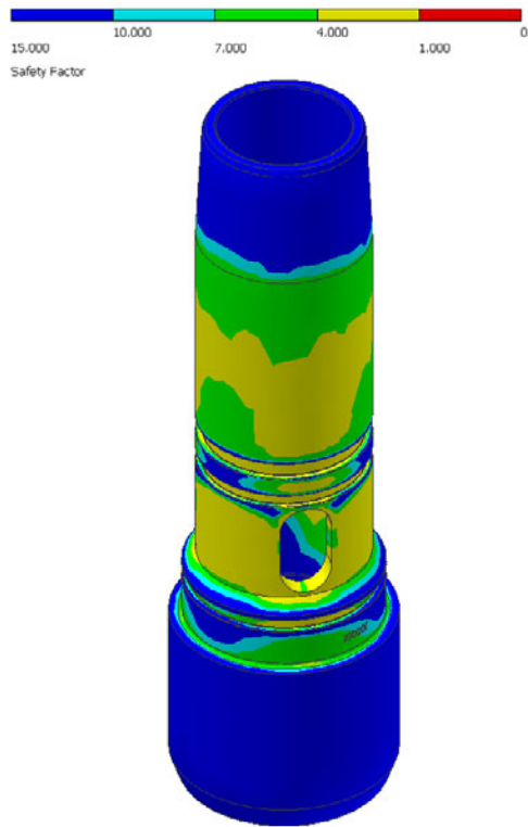
Figure 6.2 2-3/8: Safety Factor at 2200 ft-lb Cooler colours indicate higher safety factor. Red areas indicate yielding.
