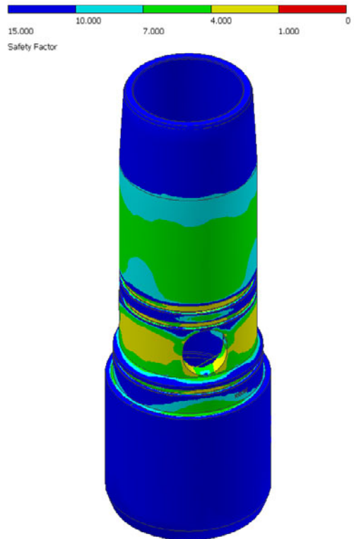
Figure 6.4 3-1/2: Safety Factor at 3910 ft-lb Cooler colours indicate higher safety factor. Red areas indicate yielding.
