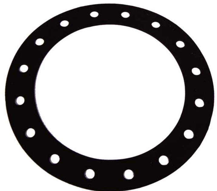
Below: Standard 8" API tank gasket for Marshhawk and Model 200 & 300 TVTH.
